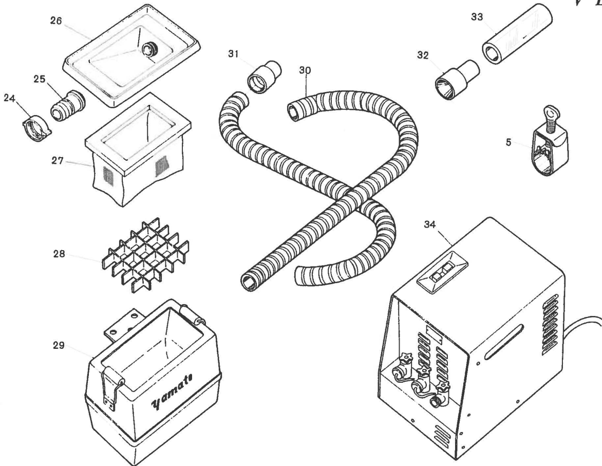
"V" DEVICE
