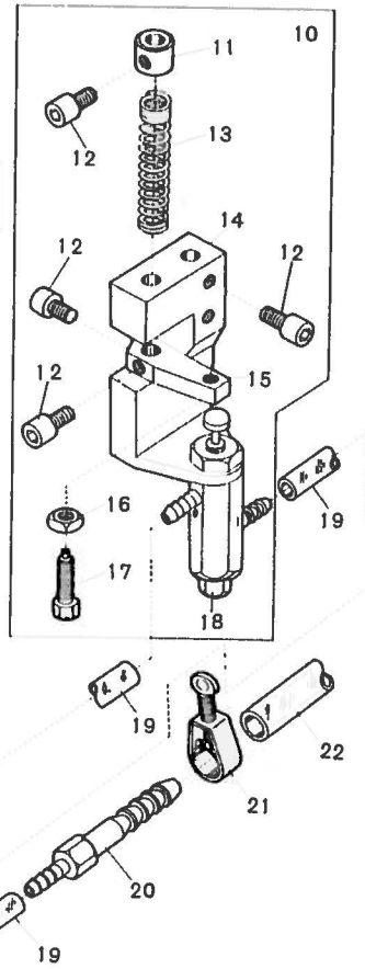
"C" DEVICE
